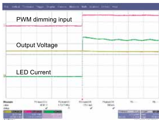
Fig. 9a: Rise time of LED Current at 40V output (5 \mu s/div)
