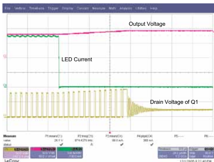
Fig. 6: Open LED Protection (20µs/div)
