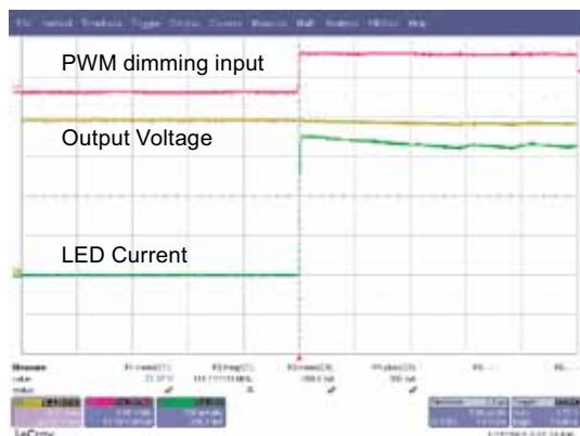
Fig. 8a: Rise time of LED Current at 80V output (5 \mu s/div)
