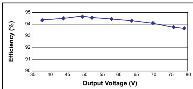
Fig. 1. Efficiency vs. Output Voltage
