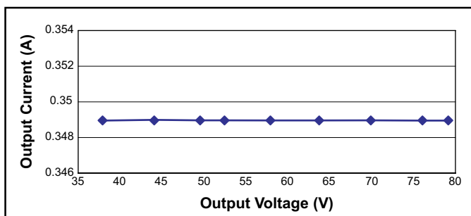
Fig. 3. Output Current vs. Output Voltage
