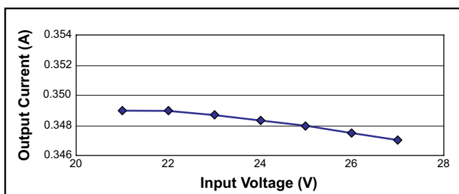
Fig. 4. Output Current vs. Input Voltage
