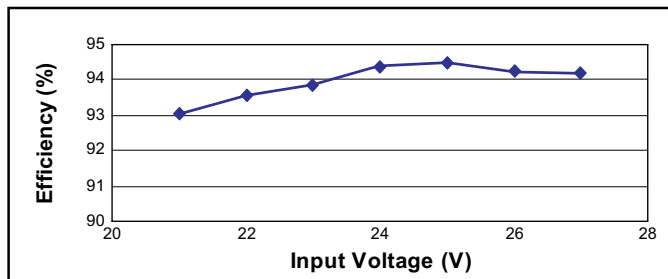
Fig. 2. Efficiency vs. Input Voltage
