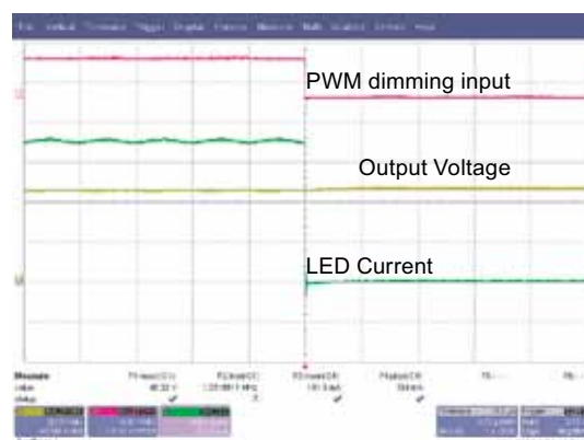
Fig. 9b: Fall time of LED Current at 40V output (5 \mu s/div)
